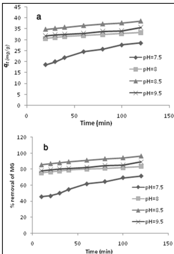
Fig. 4. Effect of contact time and initial pH on a) adsorption and b) % removal of MG onto EG-nanosheets from aqueous solutions ( T=30\text{ }^\circ\text{C} , [\text{MG}]_0=20\text{ mg L}^{-1} , EG-nanosheets=0.05 g).
