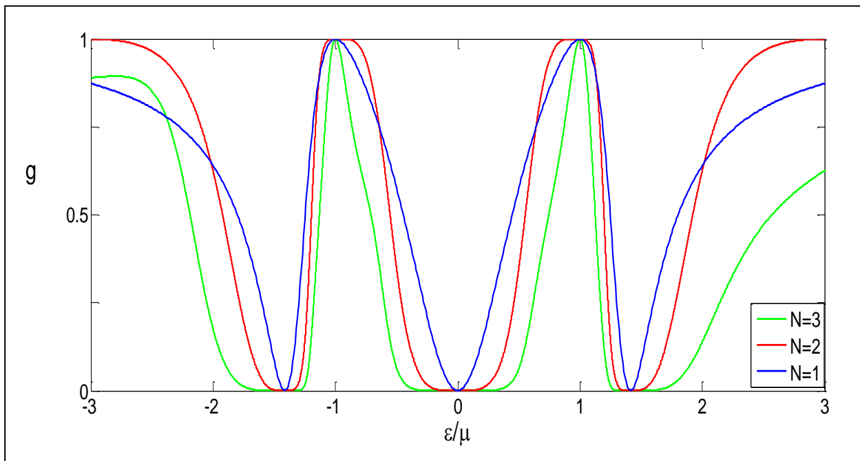
Fig. 3. Dimensionless conductance versus Fermi energy in units of \mu , for one, two and three chains for M=3 with V_c=\mu and \epsilon_0=0
