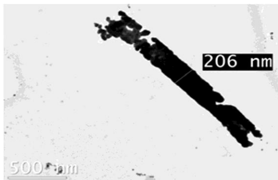
Fig.2. TEM image of a gold nanorod in the pore of the PC membrane
