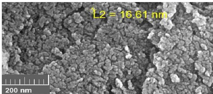
Fig. 3: FE-SEM images of nHA prepared in the presence of 0.3 g casein.
